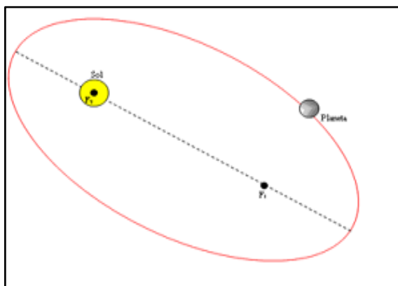
Figura 6 – Lei das órbitas (IPCC Intergovernmental Panel on Climate Change 1990)
